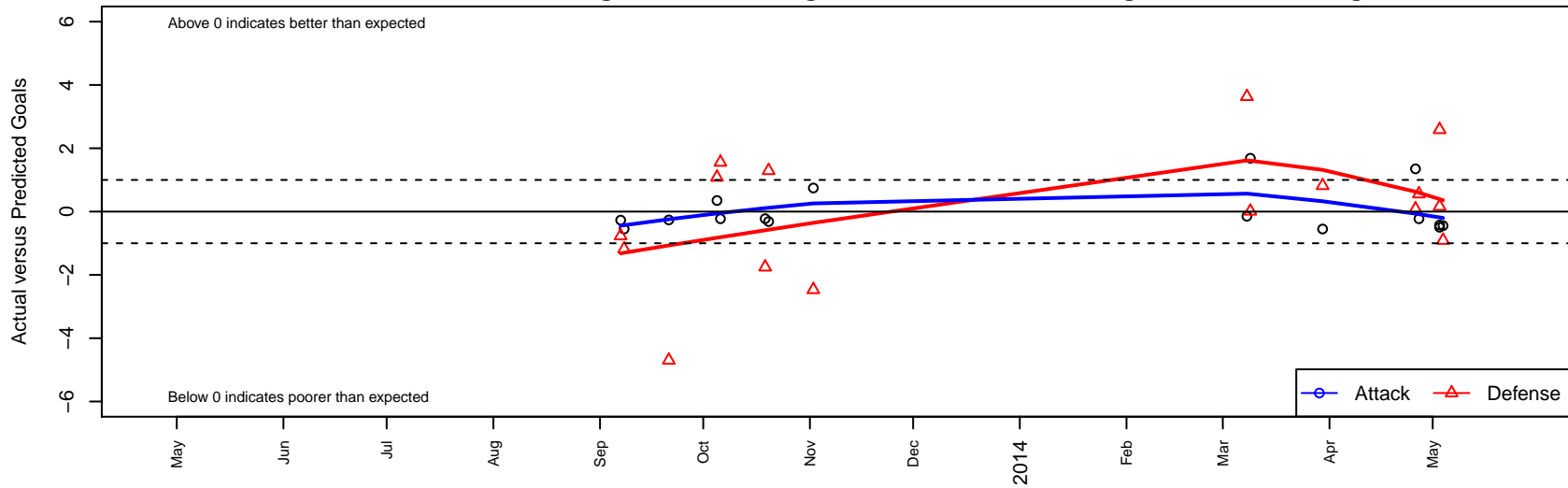
Virginia Rush SC ECNL G99 Dots are actual minus expected GF (blue circles) and GA (red triangles). Blue line is smoothed change in attack strength. Red is smoothed change in defense strength.
